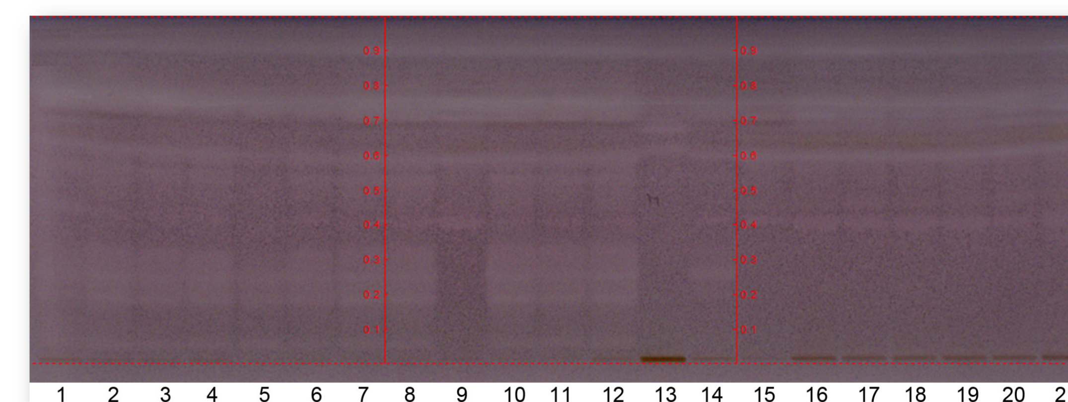
Fig. 3 Chromatograms of Salicaceae bud extract samples at white light illumination after AChE enzymatic assay.
